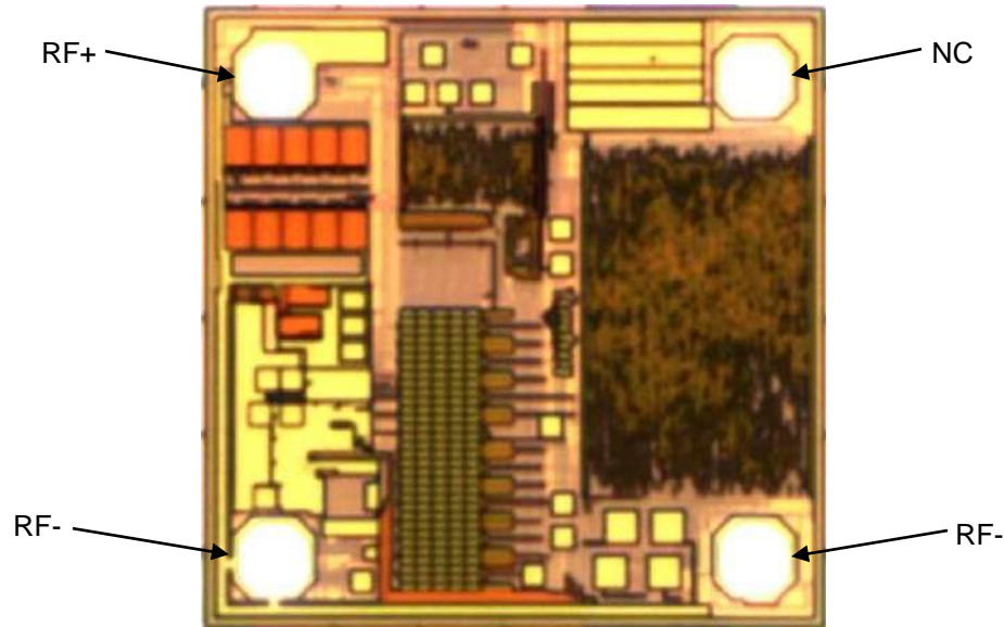
Figure 2-2 Monza 5 tag chip die orientation
