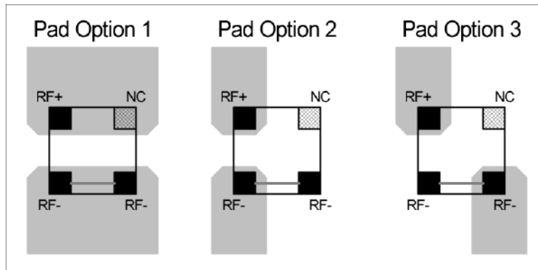
Figure 3-3: Antenna Connection Configuration Options
